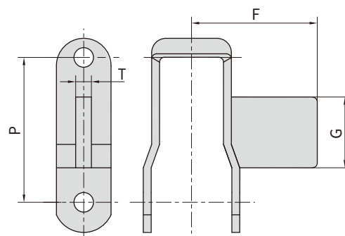
带AN附件 With AN attachments
