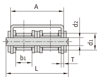
带U2部件 With U2 profile
